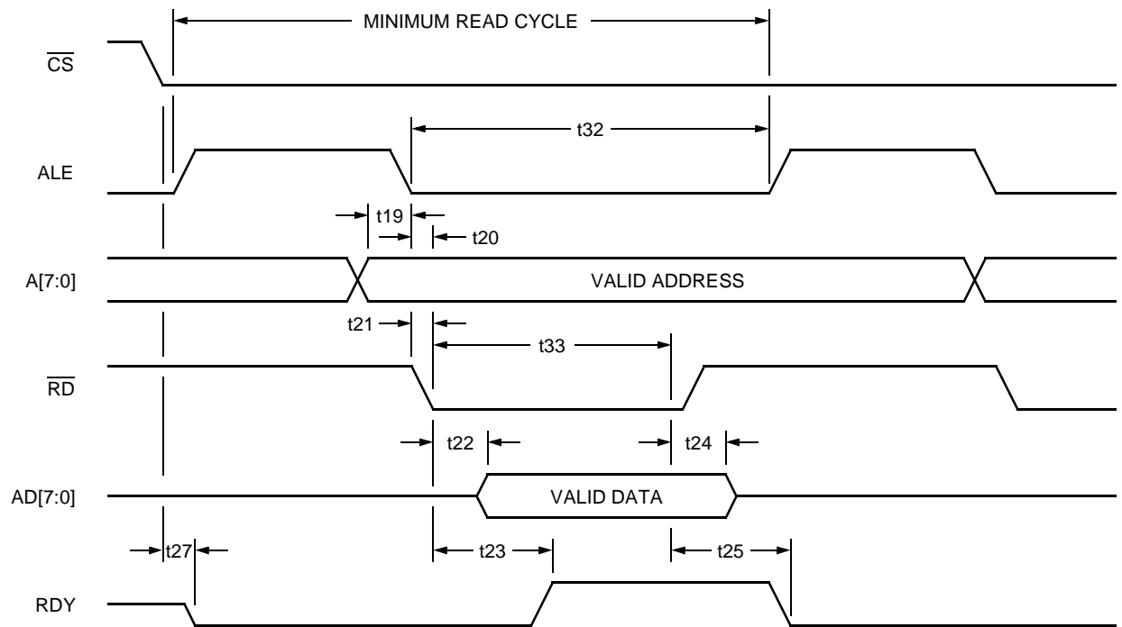
Figure 7. Mode 3—Read Cycle Timing (MPMODE = 1, MPMUX = 0)
