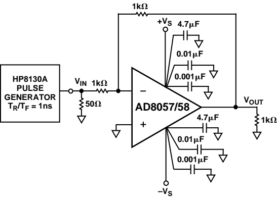
Figure 15. Test Circuit G = -1 , R_L = 1\text{ k}\Omega for Figures 16 and 17
