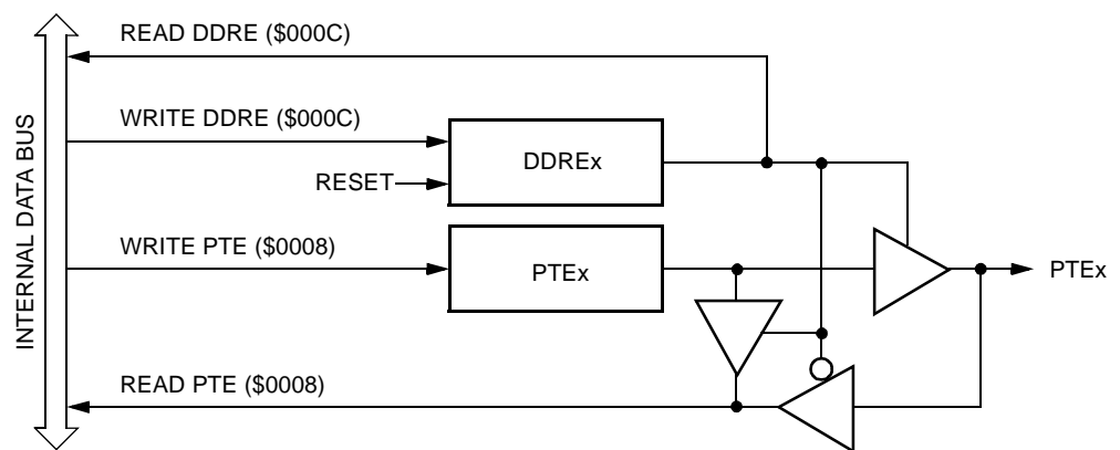
Figure 19-15. Port E I/O Circuit
