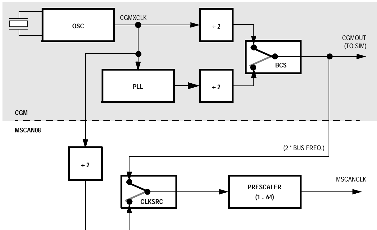
Figure 20-7. Clocking Scheme
