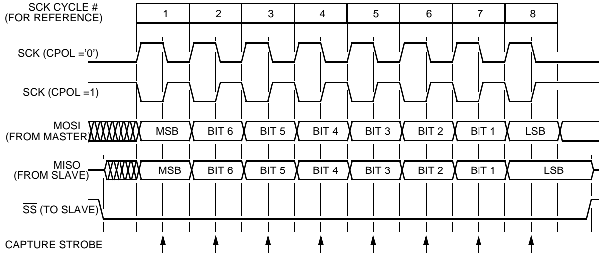
Figure 16-5. Transmission Format (CPHA = '1')
