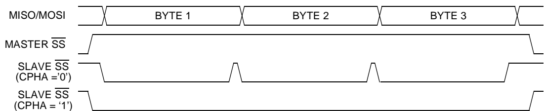
Figure 16-11. CPHA/ \overline{SS} Timing
