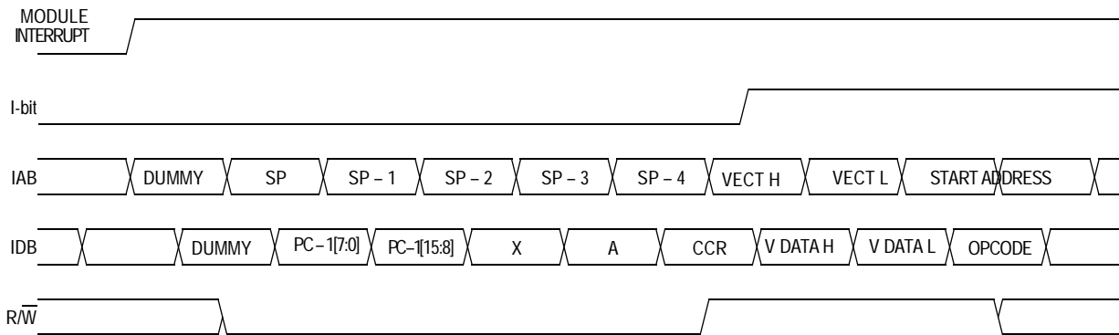
Figure 7-7. Interrupt Entry
