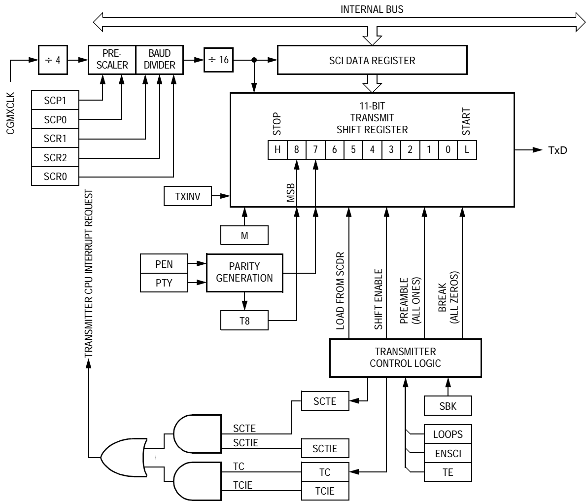
Figure 15-4. SCI Transmitter
