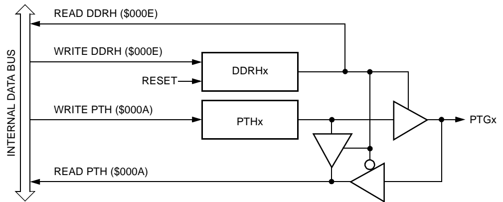
Figure 19-24. Port H I/O Circuit
