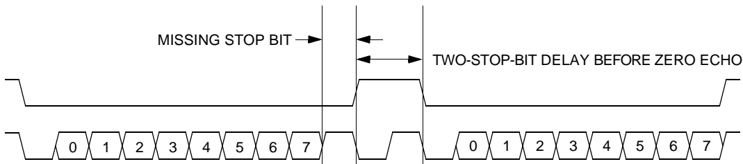
Figure 11-5. Break Transaction
