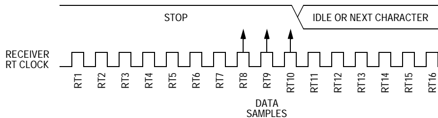
Figure 15-10. Fast Data
