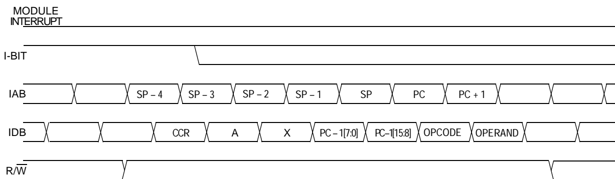
Figure 7-8. Interrupt Recovery
