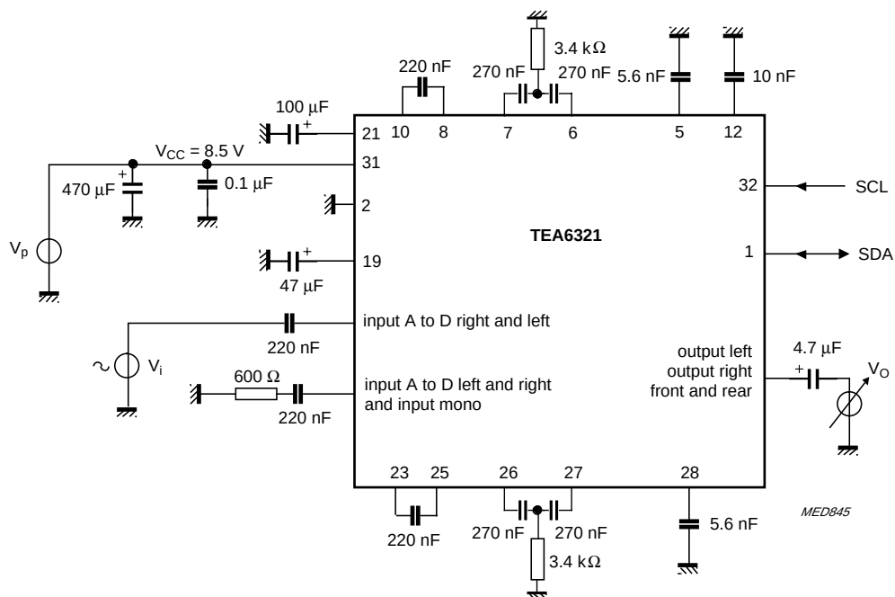
Fig.15 Test circuit for channel separation ( \alpha_{CS} ).
