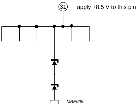
Fig.30 Pin 31: supply voltage.
