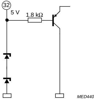
Fig.31 Pin 32: SCL (I²C-bus clock).
