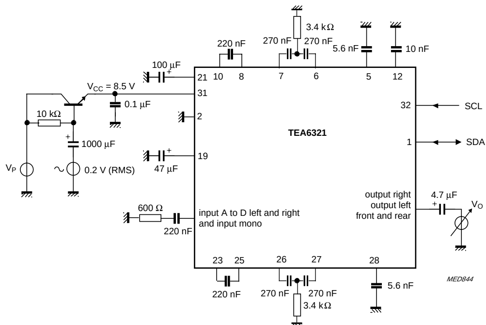
Fig.14 Test circuit for power supply ripple rejection (RR).
