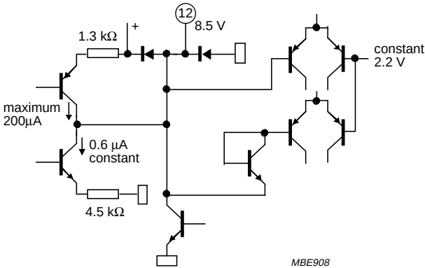
Fig.28 Pin 12: mute control.
