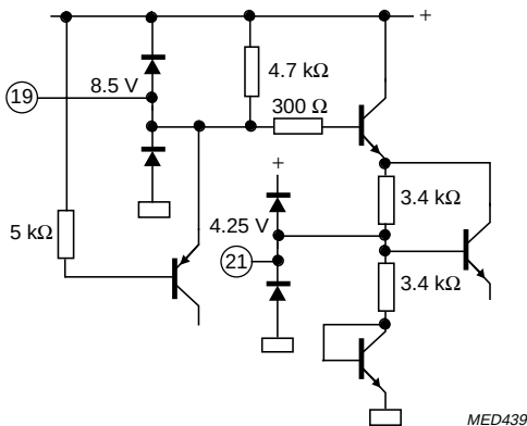
Fig.29 Pin 19: filtering for supply; pin 21: reference voltage.
