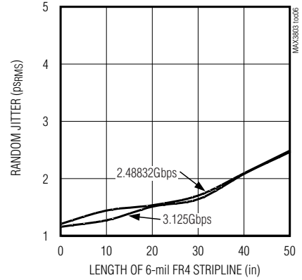
RANDOM JITTER vs. LENGTH (IN± = 800mVp-p, PATTERN = K28.7)
