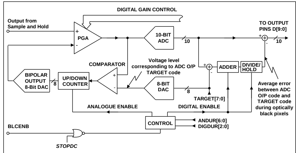
Figure 15 Basic DC Offset Correction Block Diagram
