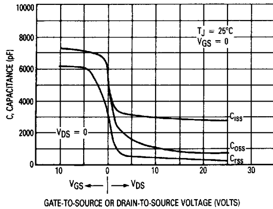
Figure 11. Capacitance Variation
