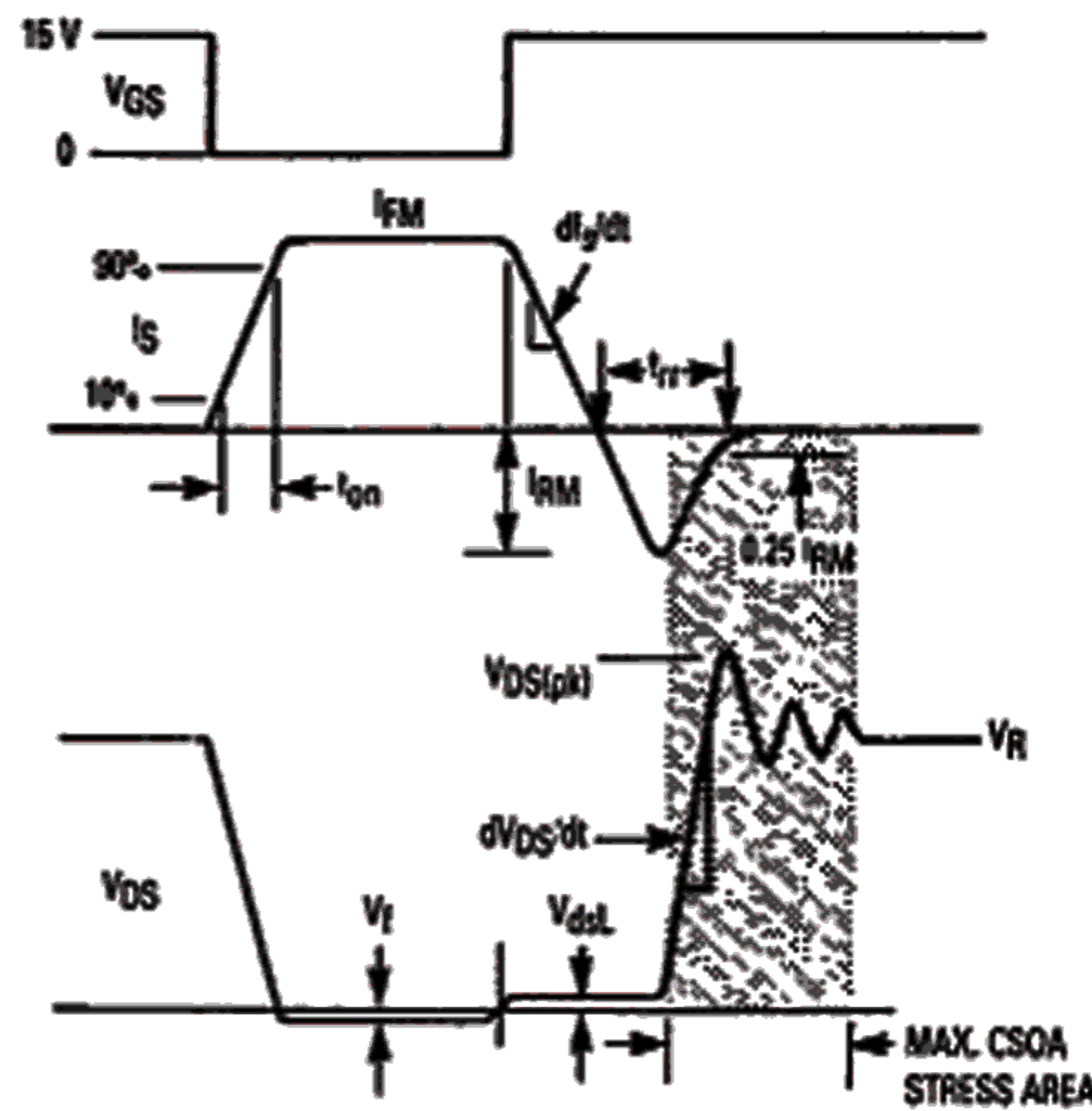
Figure 11. Commutating Waveforms
