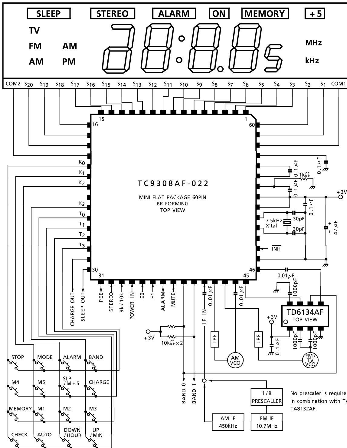
TC9308AF-022 Layout (With prescaler : TD6134AF)
