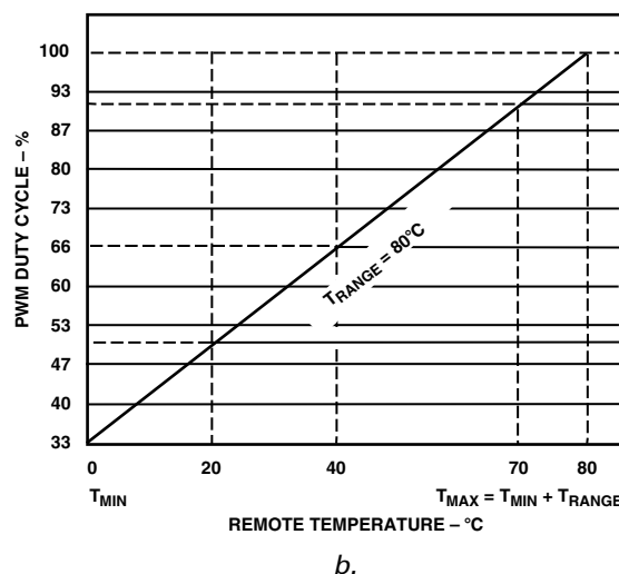
Figure 13. Max Speed Calculated by Local and Remote Temperature Control Loops Drives Fans
