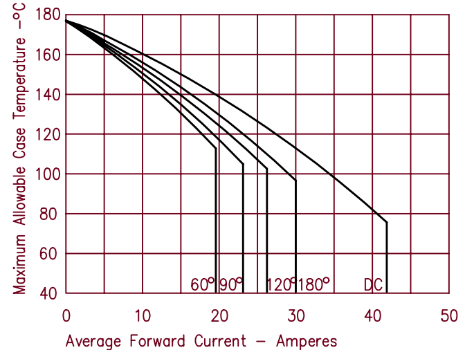
Figure 5 Forward Current Derating – Reverse Polarity – Per Leg
