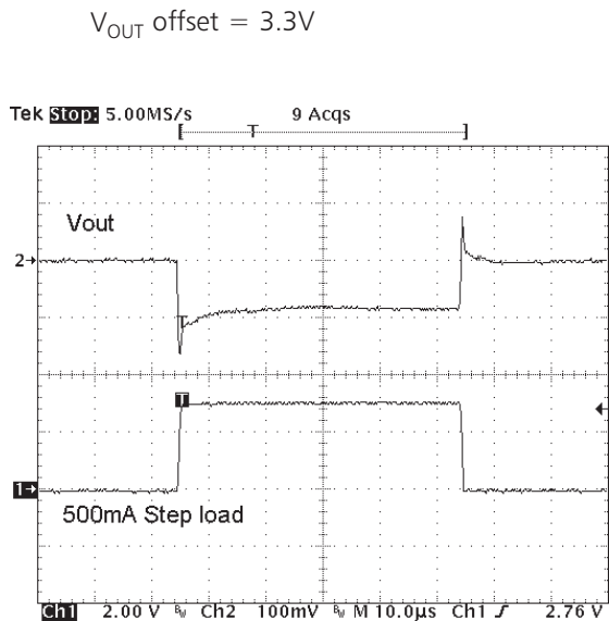
Figure 10. Load Step Response.
