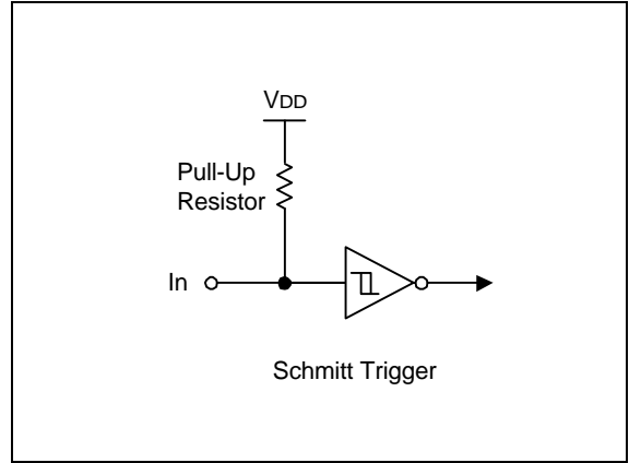
Figure 1-8. Pin Circuit Type B
