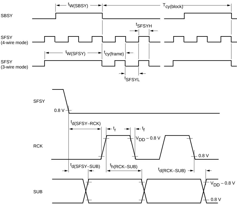
Fig.31 Subcode interface timing diagram.
