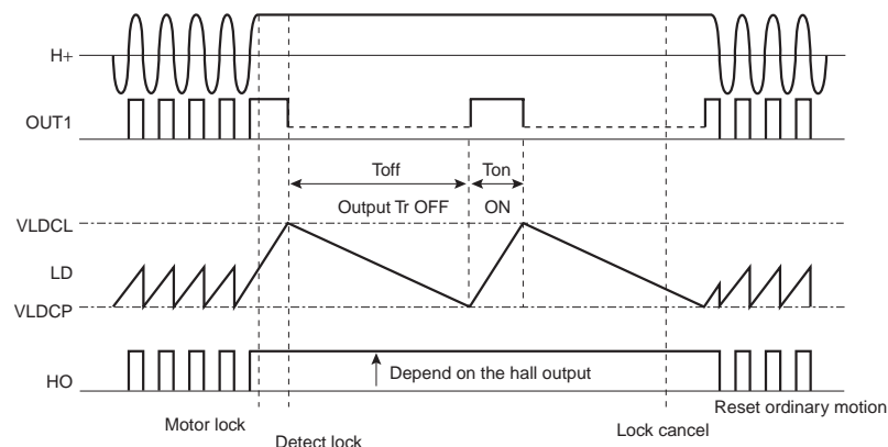
Fig.4 Timing chart
