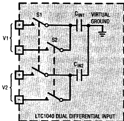
Figure 2. Dual Differential Equivalent Input Circuit
