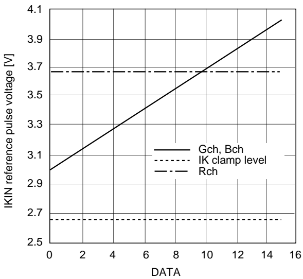
G-CUTOFF, B-CUTOFF
