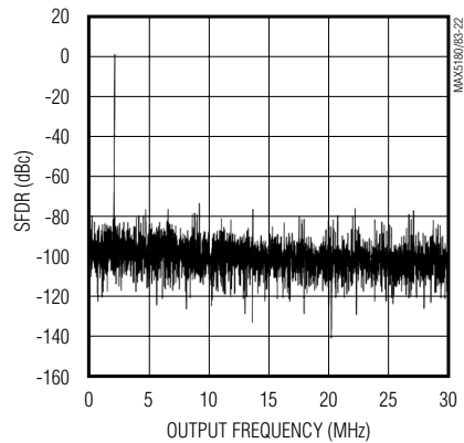
SPURIOUS-FREE DYNAMIC RANGE vs. OUTPUT FREQUENCY
