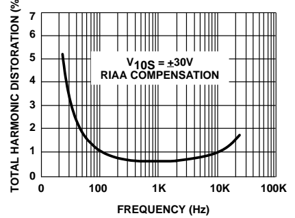
Distortion vs Frequency VO = 1VRMS
