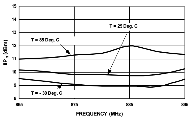
IIP 3 vs. Temperature I_{DD} = 4.9\text{ mA} , R_{F_{IN}} = -27\text{ dBm}
