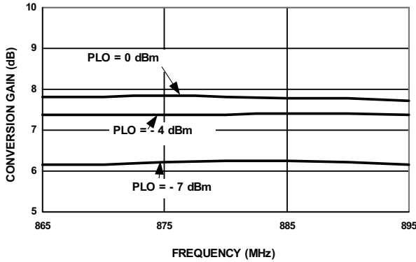
Conversion Gain vs. LO Power
