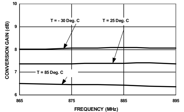
Conversion Gain vs. Temperature I_{DD} = 4.9\text{ mA} , R_{F_{IN}} = -27\text{ dBm}
