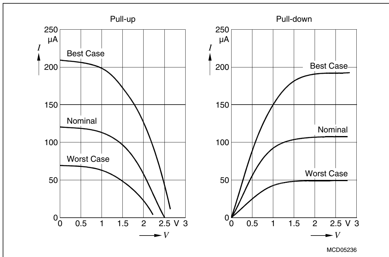
Figure 23 Pull-Up/Pull-Down Characteristics of Class B Pins
