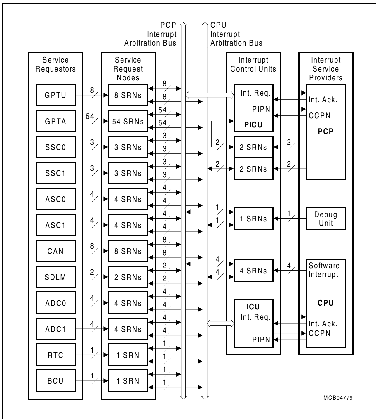
Figure 16 Block Diagram of the TC1775 Interrupt System
