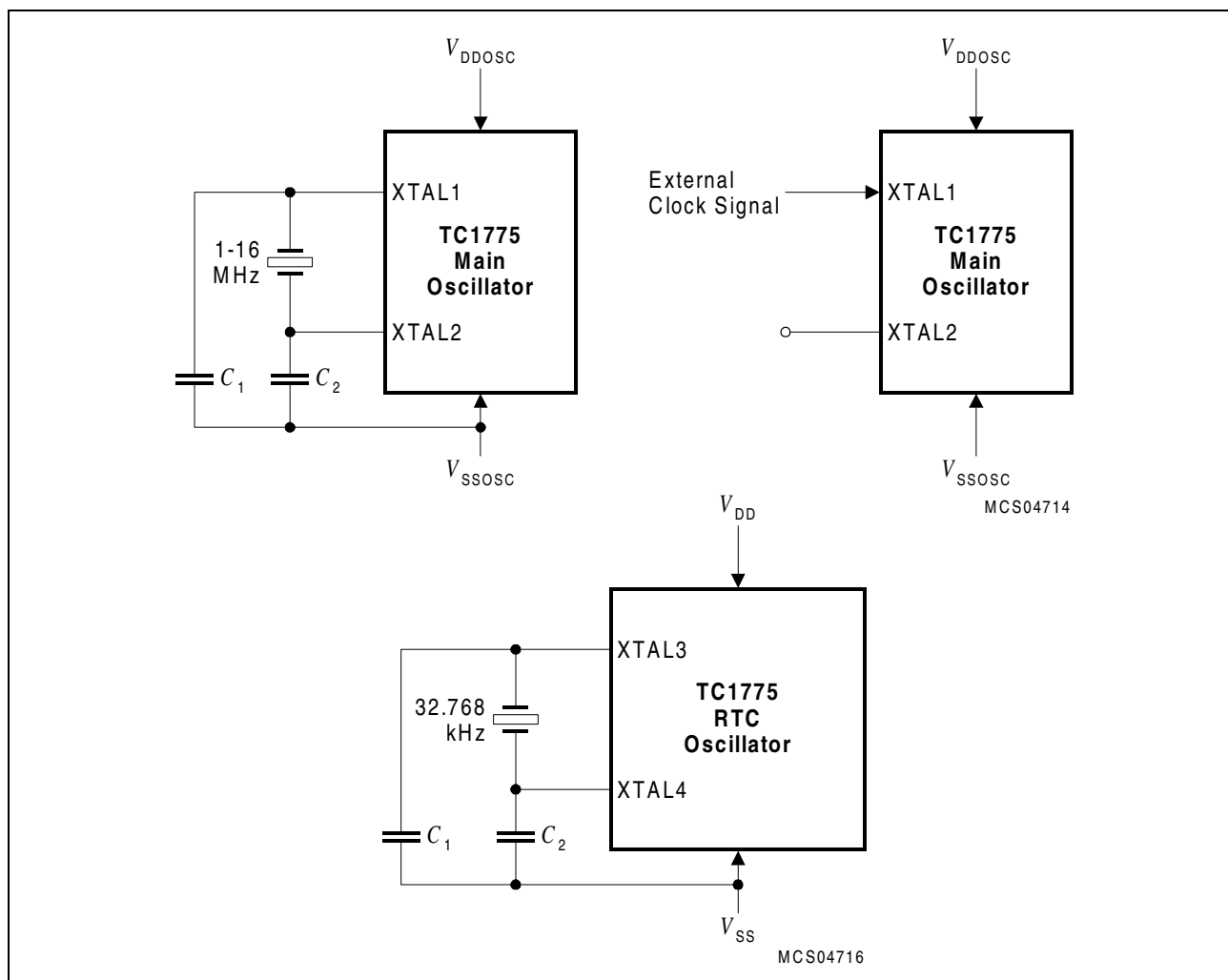
Figure 19 Oscillator Circuitries
