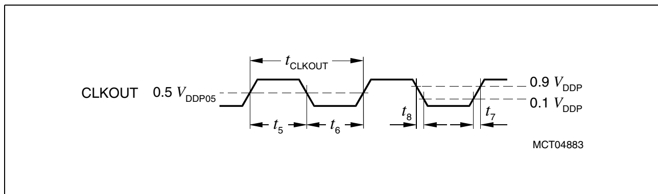
Figure 30 CLKOUT Output Clock Timing
