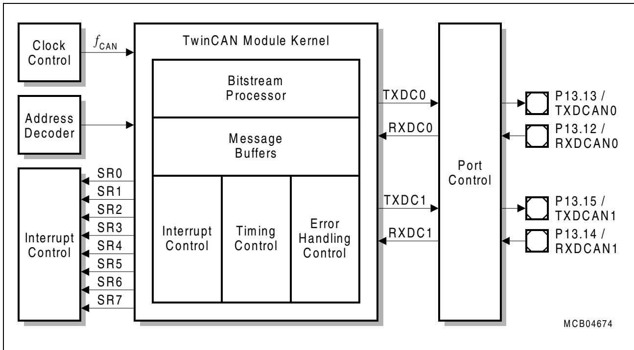
Figure 7 General Block Diagram of the TwinCAN Module
