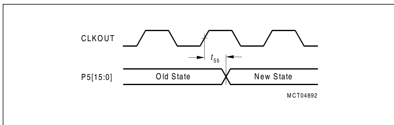
Figure 40 Port 5 Timing
