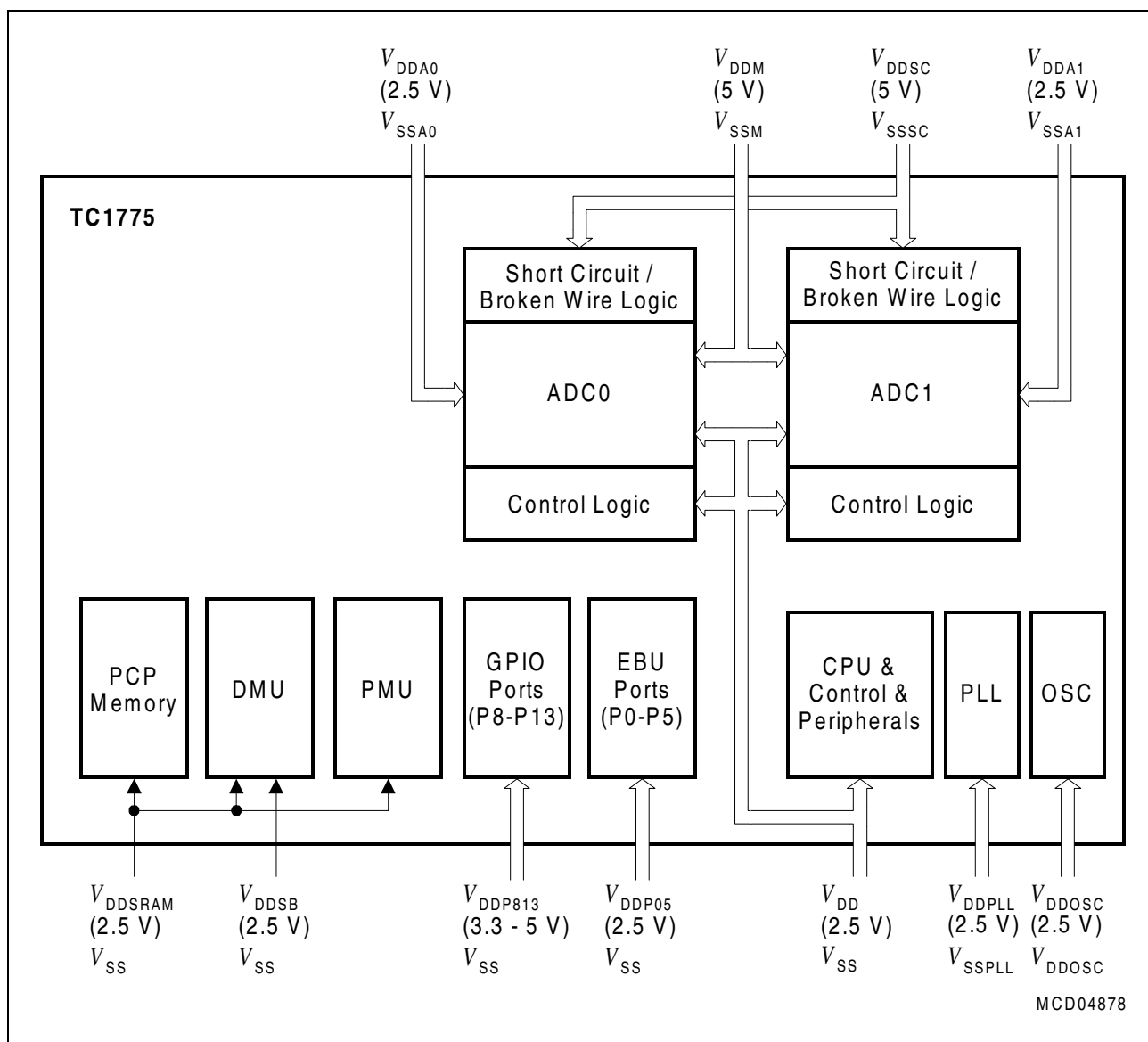
Figure 20 TC1775 Power Supply Concept
