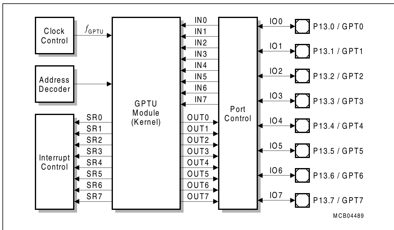
Figure 9 General Block Diagram of the GPTU Interface
