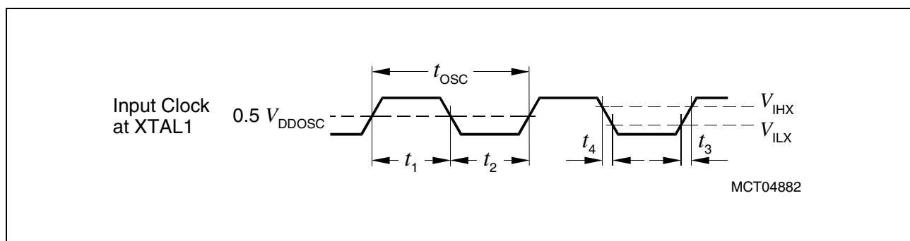
Figure 29 Input Clock Timing
