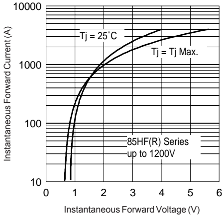
Fig. 11 - Forward Voltage Drop Characteristics (up to 1200V)
