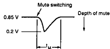
Figure 4. Mute timing
