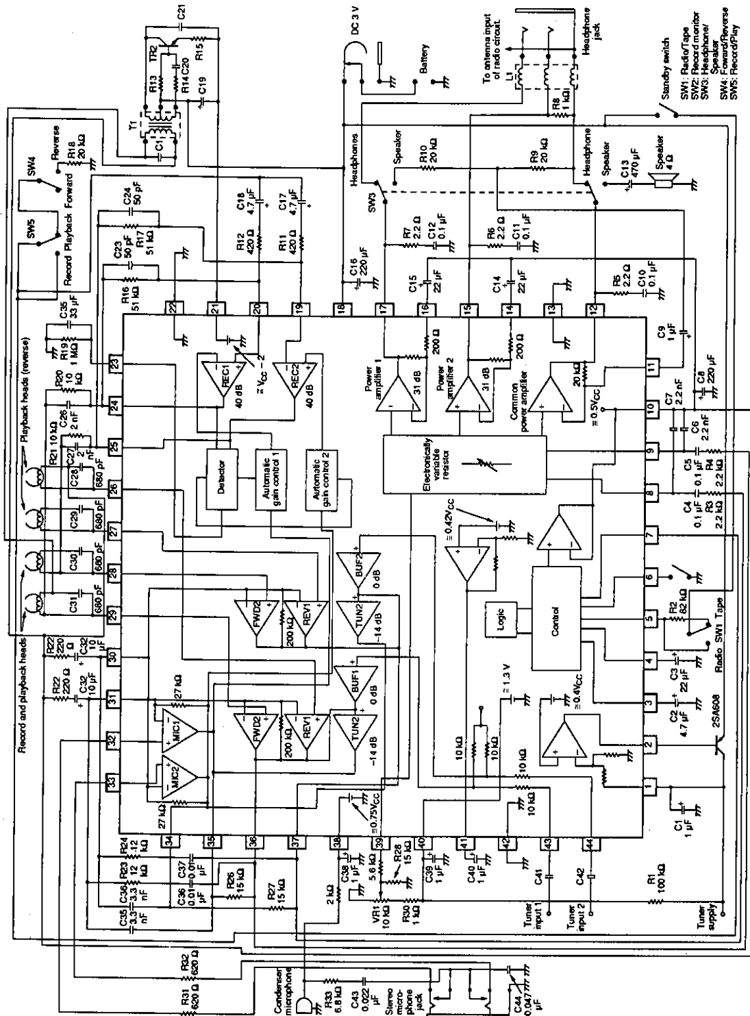
Figure 10. Typical application
