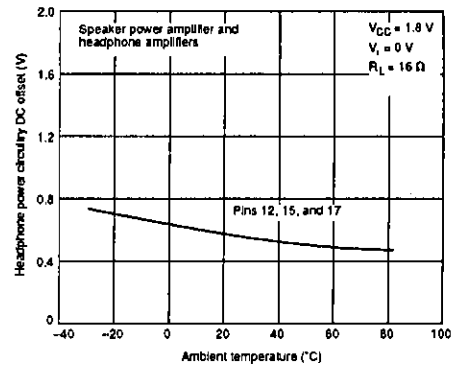
Amplifier DC offset vs. ambient temperature (5)
