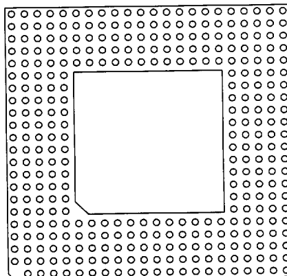
339 Pins 2
