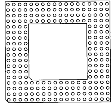
224 Pins 4 Without Window FP 05
