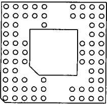
73 Pins 19
