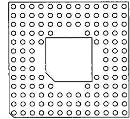
132 Pins 57
