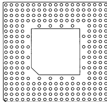
257 Pins 9 Without Window FP 08
