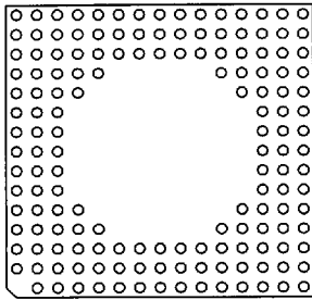
155 Pins 45
