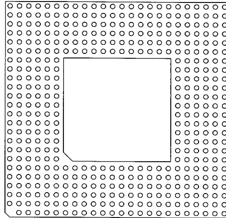
431 Pins 2 DEC AXP210G4A & AXP21064
