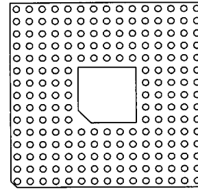
200 Pins 60
