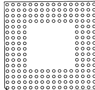
192 Pins 19
