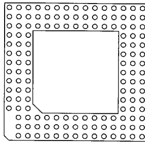
141 Pins 27 Without Window FP28
