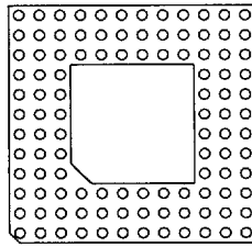
108 Pins 4 Without Window FP 05
