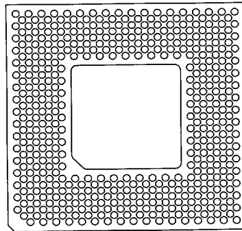
431 Pins B3 Without Window FP A9
