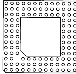
119 Pins 19 Without Window FP 20
