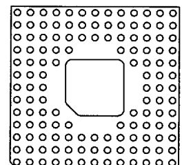
132 Pins 93 Without Window FP 47
