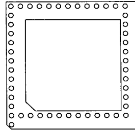
49 Pins 18 Without Window FP 19
