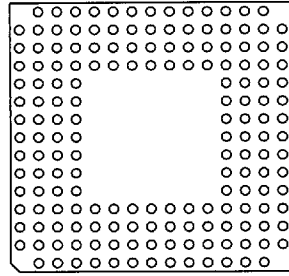
172 Pins 47
