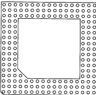
169 Pins 8 Without Window FP 18 Intel i486
