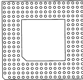
223 Pins 8 Without Window FP 13
