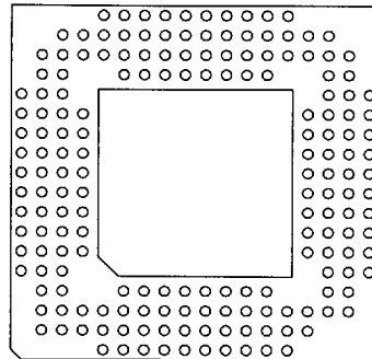
180 Pins 27 Without Window FP 25
