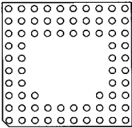
72 Pins 4
