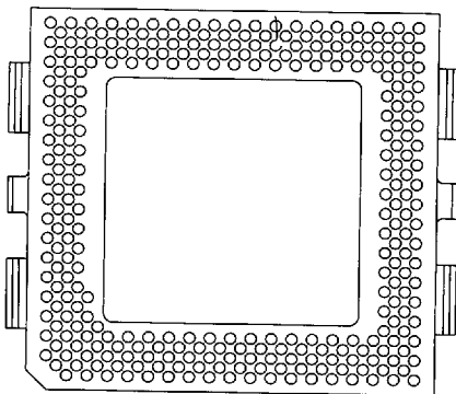
296 Pins B4* With Heatsink Tabs Intel Pentium™ P54C
