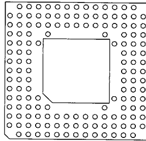
149 Pins 17 Without Window FP18
