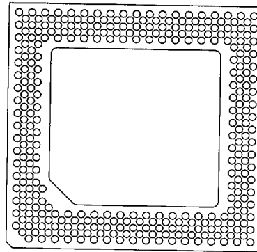
296 Pins A3 Without Window FP A2 Intel Pentium™ P54C
