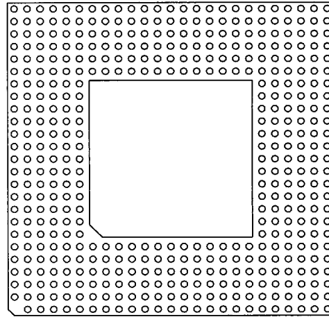
455 Pins 2
