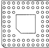
68 Pins 5 Without Window FP06 Motorola 68000
