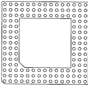
144 Pins 23 Without Window FP24
