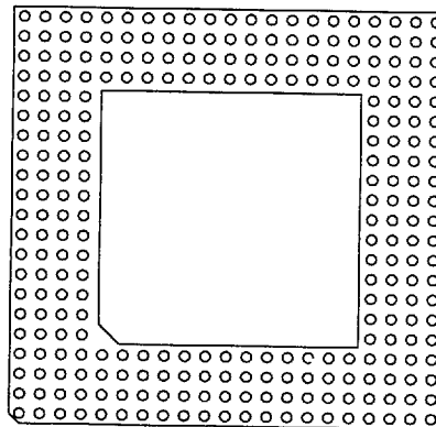
272 Pins 13 Without Window FP 02
