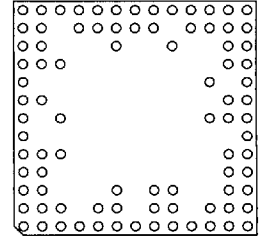
88 Pins 43
