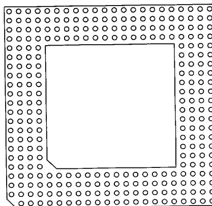
287 Pins 6 Without Window FP 05
