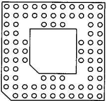
83 Pins 13
