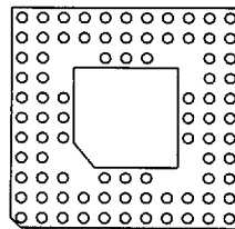
85 Pins 7
