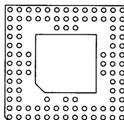
100 Pins 2A Without Window FP 98
