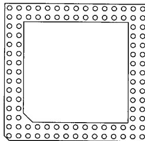
104 Pins 42 Without Window FP43
