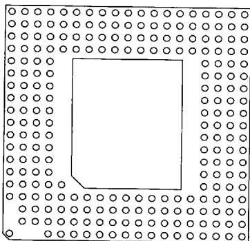
237 Pins 25 Without Window FP 27 Intel P24CT
