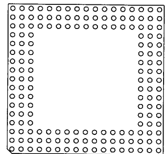
168 Pins 11
