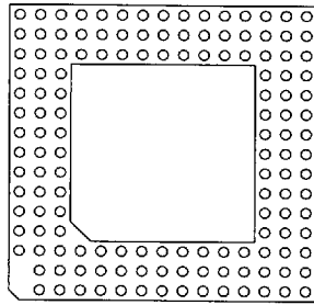
142 Pins 25 Without Window FP26
