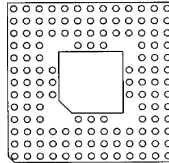
132 Pins 6 Without Window FP 07
