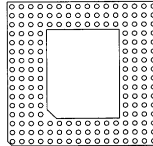
176 Pins 20 Without Window FP 18
