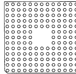
160 Pins 56
