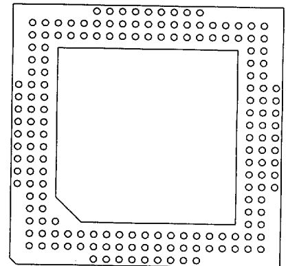
173 Pins 14
