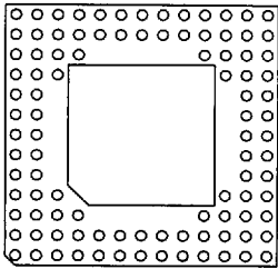
100 Pins 23 Without Window FP 24
