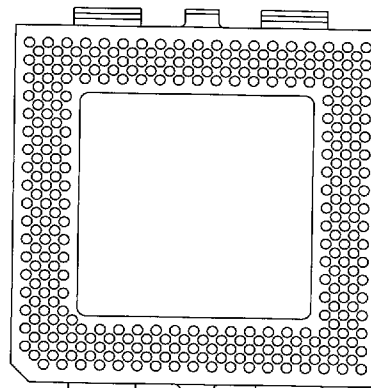
320 Pins B5* With Heatsink Tabs Intel Pentium™ P54CM
