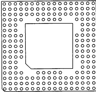
192 Pins 56 Without Window FP 52
