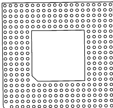
299 Pins 2 Without Window FP 07
