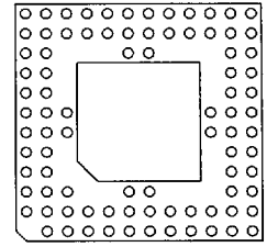
88 Pins 8 Without Window FP 09
