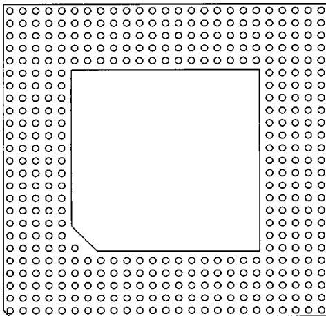
401 Pins 3 Without Window FP 04
