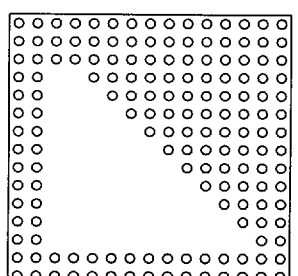
160 Pins 14
