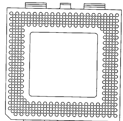
321 Pins B6* With Heatsink Tabs Intel Pentium™ P55CM
