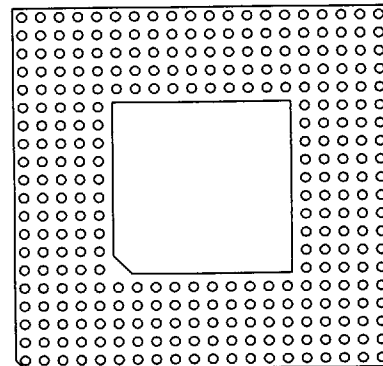
300 Pins 3 Without Window FP 09
