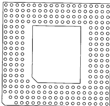
238 Pins 16 Without Window FP 18 Intel P24T
