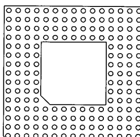
176 Pins 12
