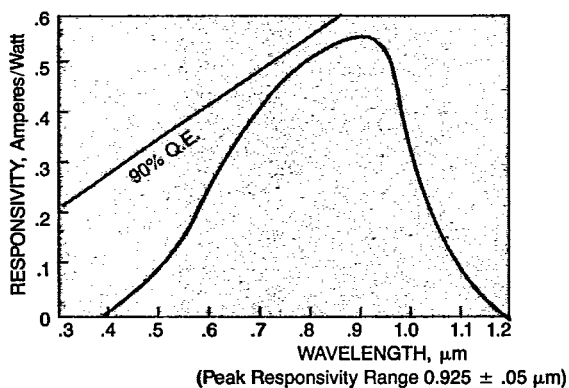
Typical Responsivity vs. Wavelength
