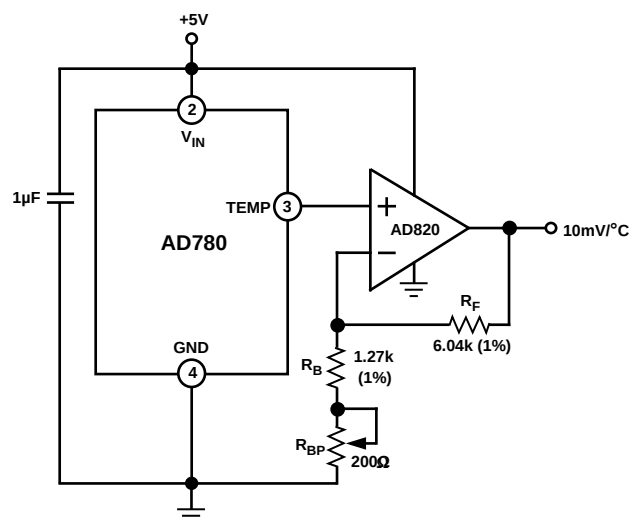
Figure 9. Differential Temperature Transducer
