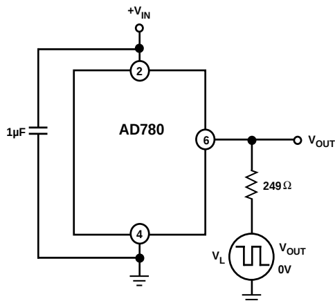
Figure 12a. Transient Resistive Load Test Circuit
