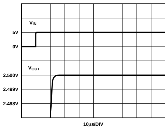
Figure 11. Turn-On Settling Time Performance
