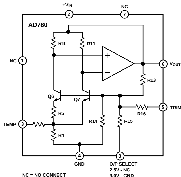
Figure 1. Schematic Diagram
