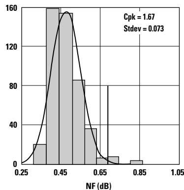
Figure 4. NF @ 2 GHz, 3 V, 60 mA. USL = 0.9, Nominal = 0.49
