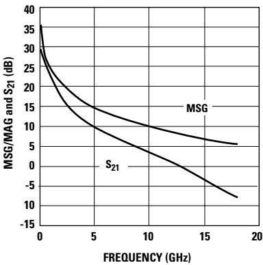
Figure 28. MSG/MAG and |S_{21}|^2 vs. Frequency at 4V, 60 mA.
