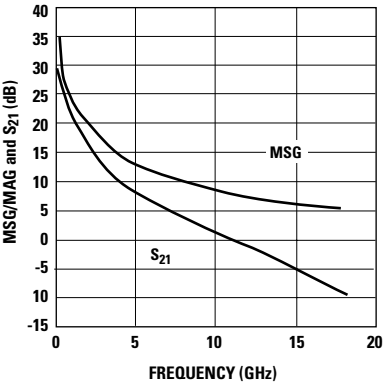
Figure 27. MSG/MAG and |S_{21}|^2 vs. Frequency at 3V, 80 mA.
