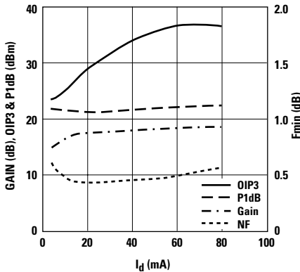
Figure 21. OIP3, P1dB, Gain and Fmin vs. Ids at 4V @ 2 GHz.
