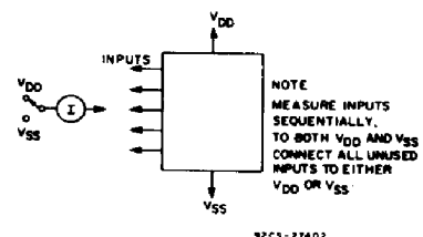
Fig. 12 – Input current.
