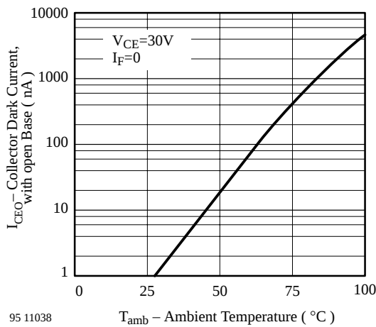
Figure 9. Collector Dark Current vs. Ambient Temperature
