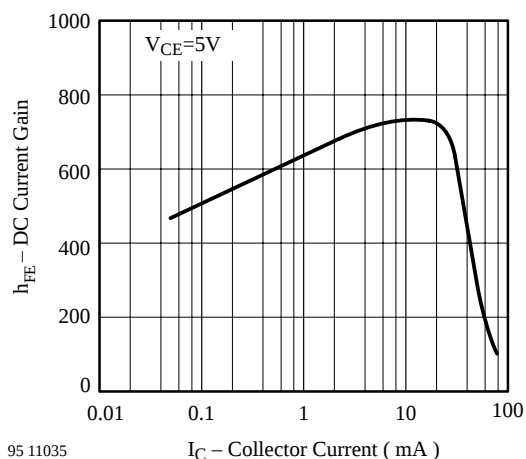
Figure 18. DC Current Gain vs. Collector Current
