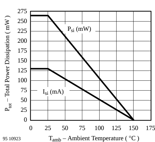
Figure 1. Derating diagram
