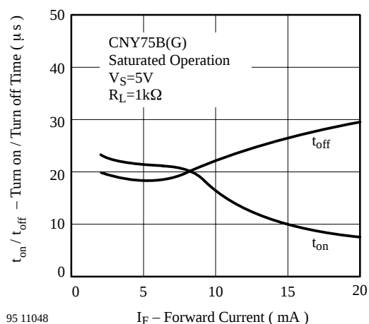
Figure 23. Turn on / off Time vs. Forward Current
