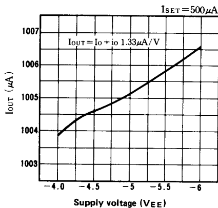
Output current vs. Supply voltage ( V_{\text{EE}} )
