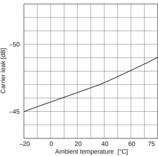
Carrier leak 3.58MHz temperature characteristics
