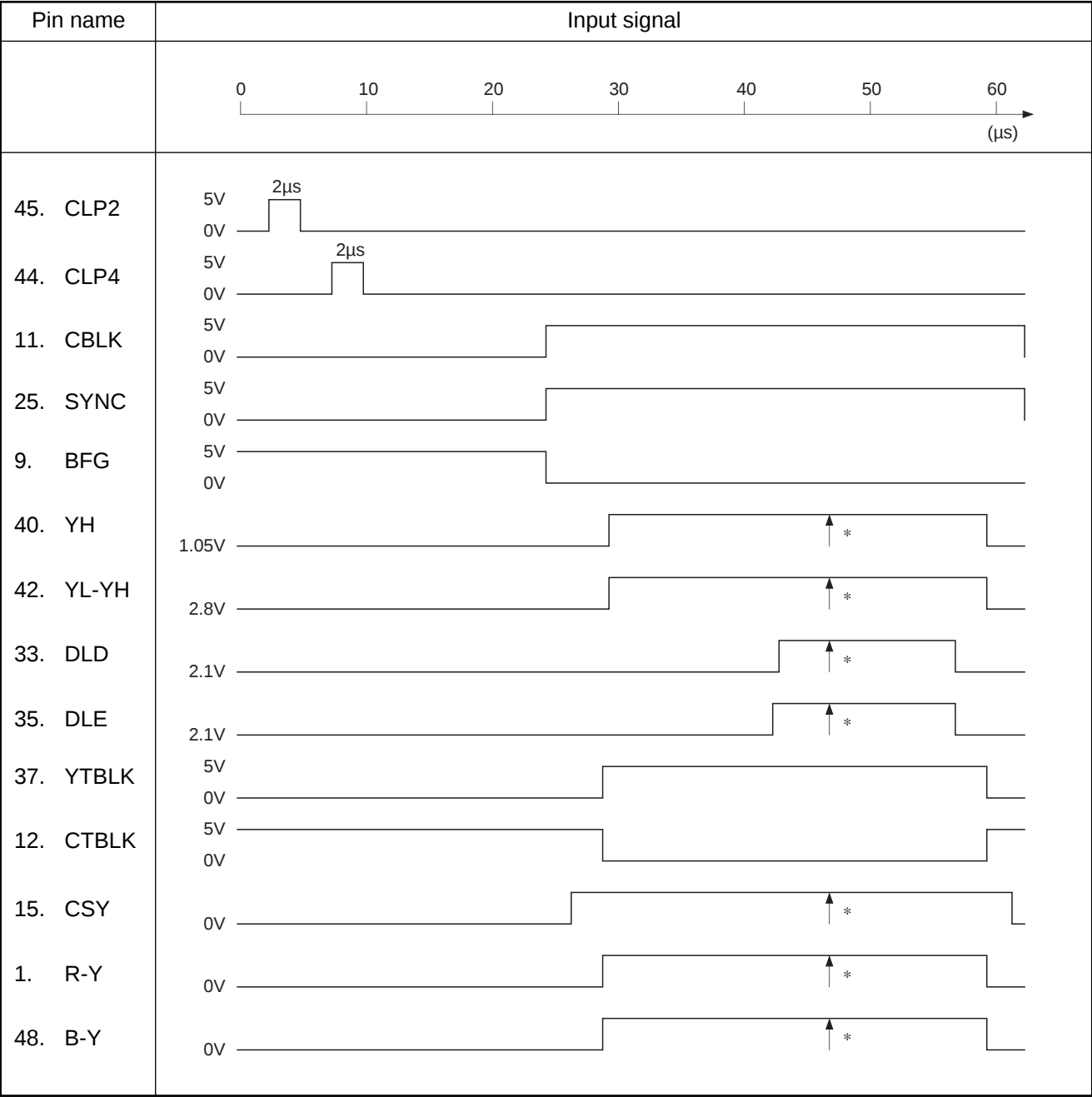
Input Signal Timing Chart
