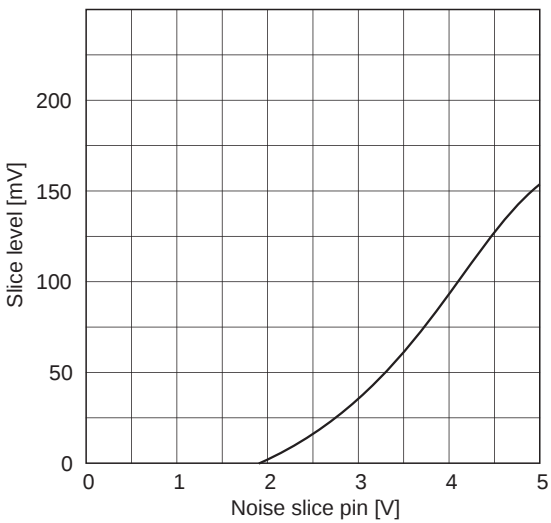
SHP noise slice characteristics
