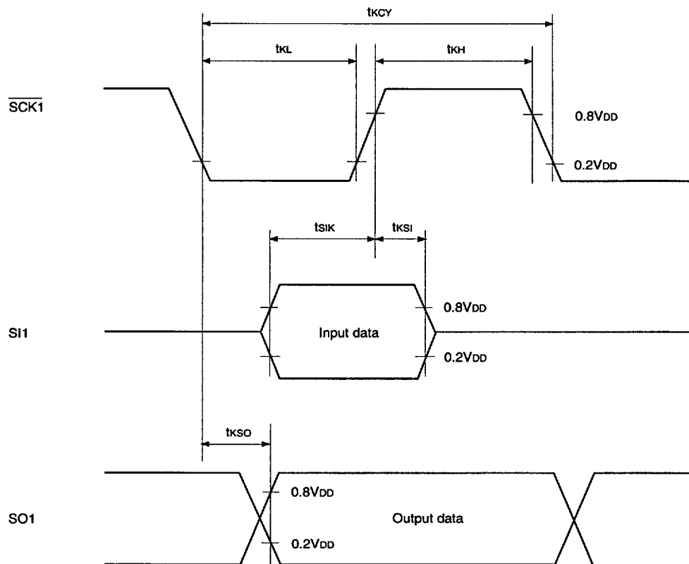
Fig. 5. Serial transfer CH1 timing
