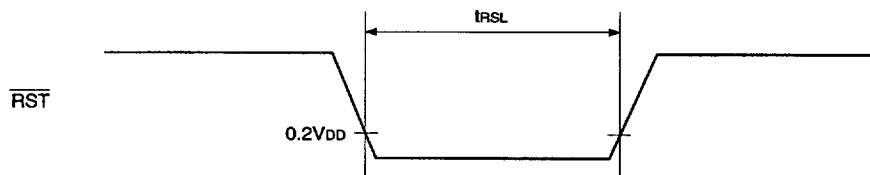
Fig. 8. Reset input timing
