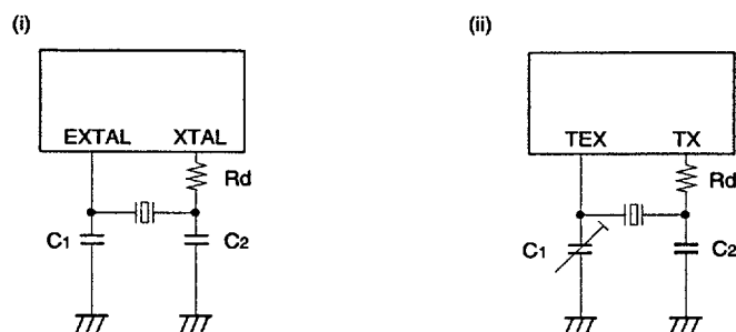
Fig. 10. Recommended oscillation circuit
