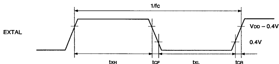
Fig. 2. Clock applied condition
