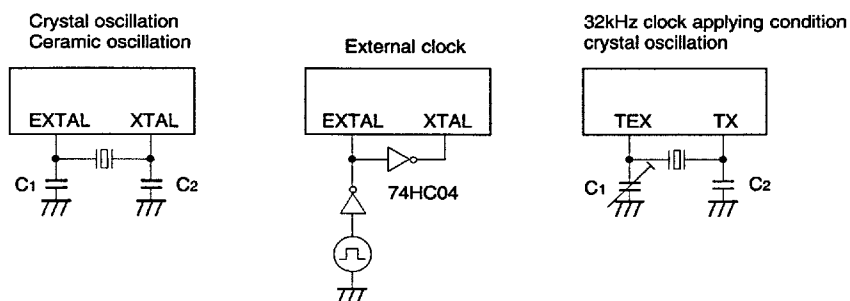
Fig. 2. Clock applied condition
