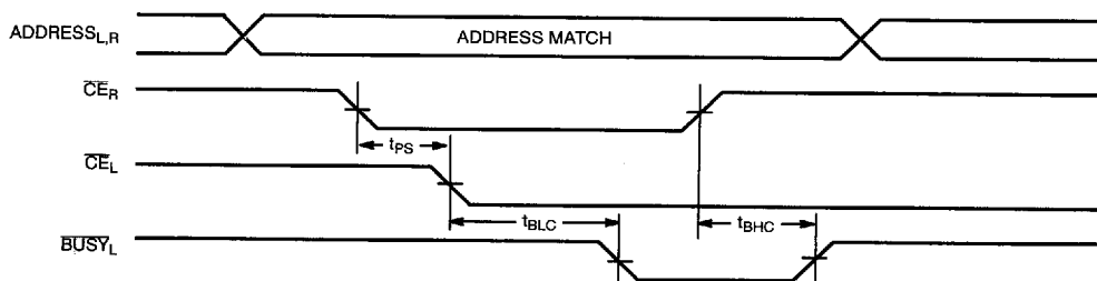
Busy Timing Diagram No. 2 (Address Arbitration) [28]
