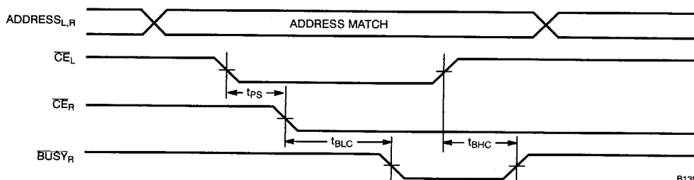
Busy Timing Diagram No. 1 (CE Arbitration) [28]
