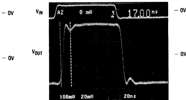
Small Signal Response
