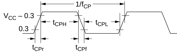
Figure 26 Oscillator Timing
