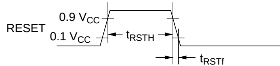
Figure 28 Reset Timing
