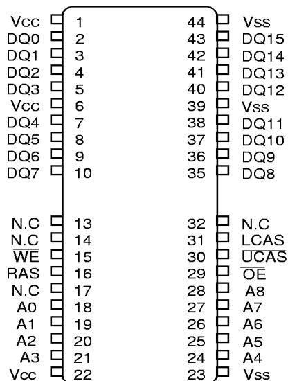
40/44Pin Plastic TSOP-II (400mil)
