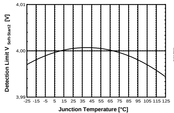
Figure 38 Detection Limit V_{Soft-Start2} vs. T_j
