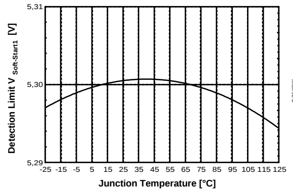
Figure 37 Detection Limit V_{Soft-Start1} vs. T_j
