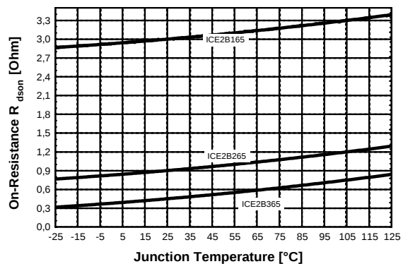
Figure 42 Drain Source On-Resistance R_{DS(on)} vs. T_j
