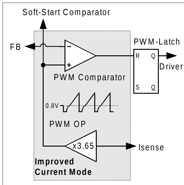
Figure 4 Current Mode
