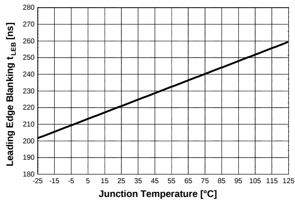
Figure 41 Leading Edge Blanking V_{CC1} vs. T_j
