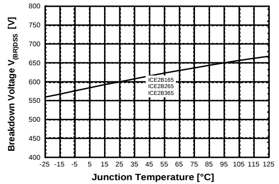
Figure 43 Breakdown Voltage V_{BR(DSS)} vs. T_j
