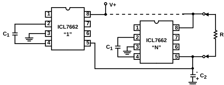
FIGURE 18. PARALLELING DEVICES
