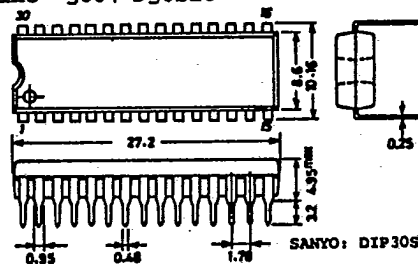
Case Outline 3061-D30SIC (unit:mm)
