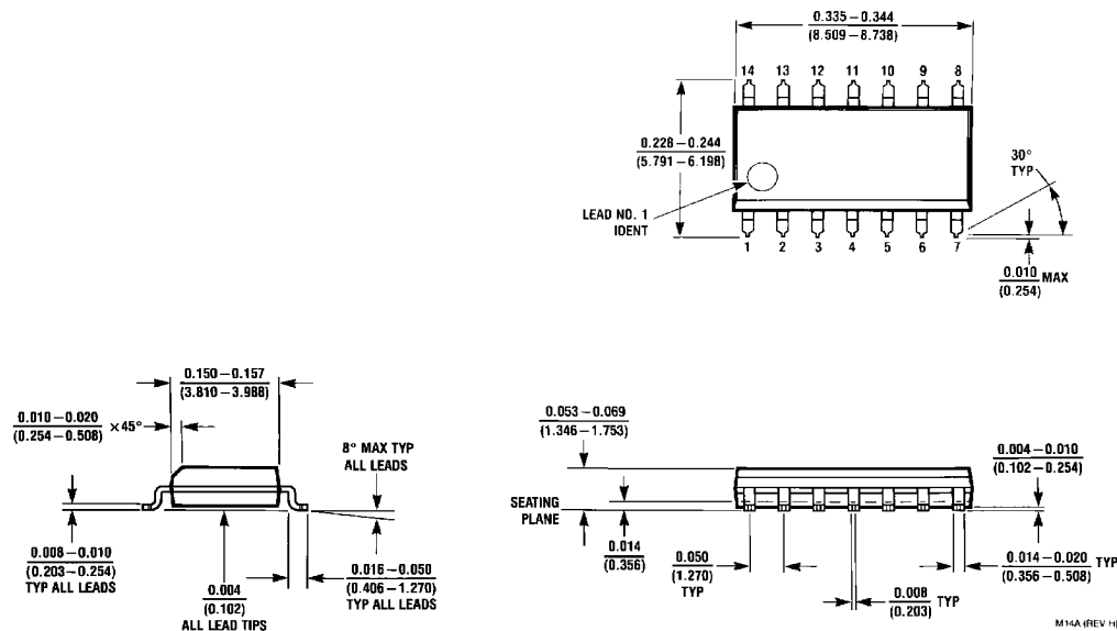
Order Number LM361M NS Package Number M14A
