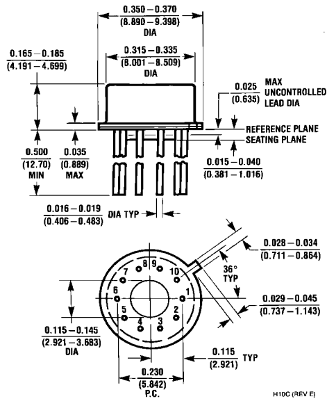
Metal Can Package (H) Order Number LM161H/883, or LM361H NS Package Number H10C
