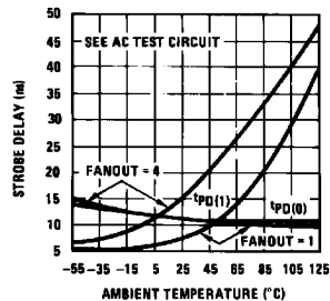
Strobe Delay vs Ambient Temperature
