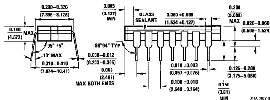
Ceramic Dual-In-Line Package (J) Order Number LM161J NS Package Number J14A
