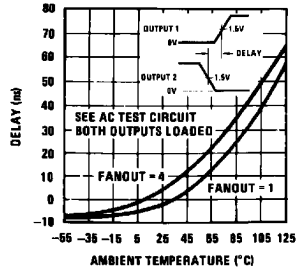
Delay of Output 1 With Respect to Output 2 vs Ambient Temperature
