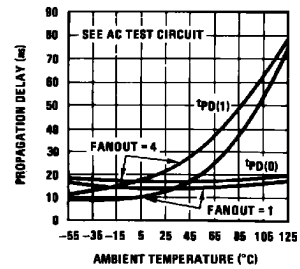
Propagation Delay vs Ambient Temperature
