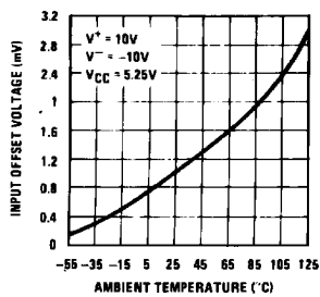
Offset Voltage
