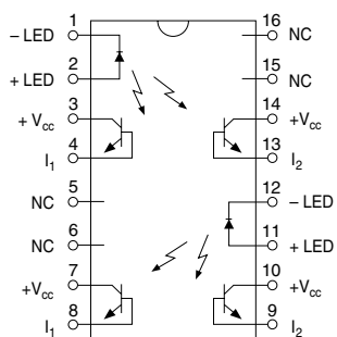
LOC210 Pinout
