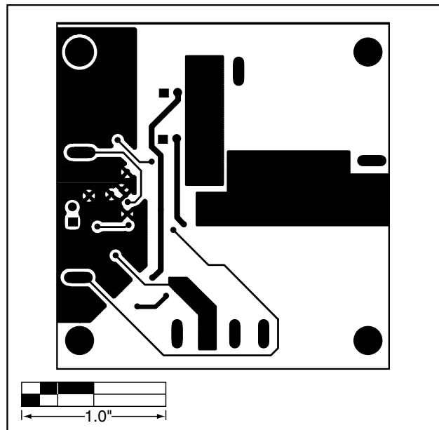
Figure 4. MAX1747 EV Kit PC Board Layout—Solder Side
