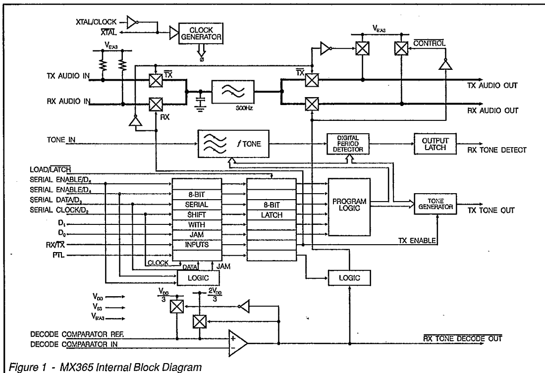
Figure 1 - MX365 Internal Block Diagram
