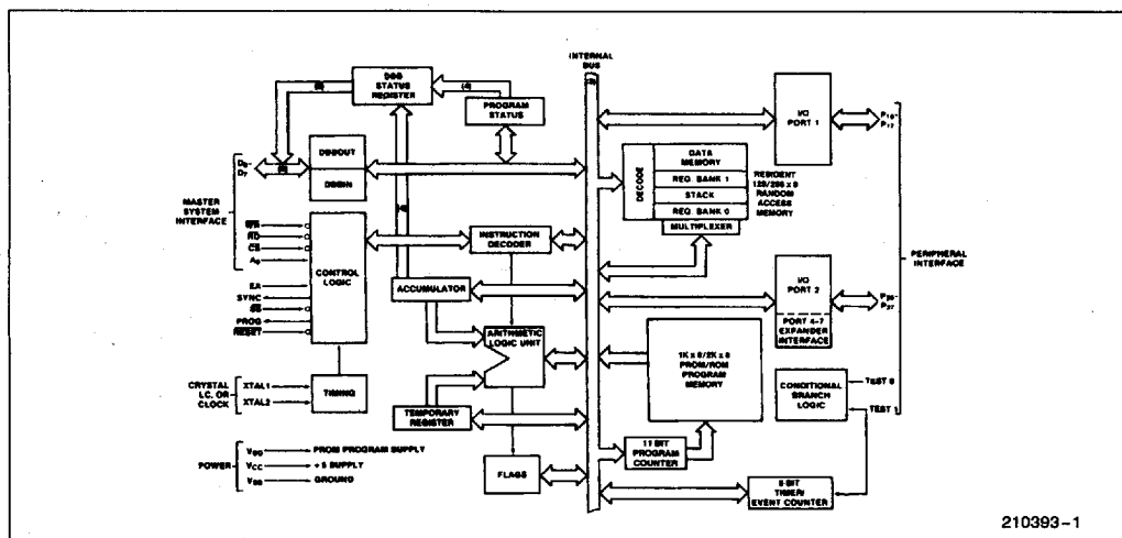
Figure 3. Block Diagram
