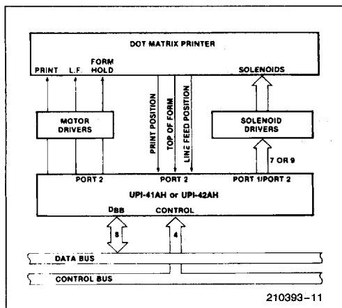
Figure 8. UPI-41AH/42AH 80-Column Matrix Printer Interface
