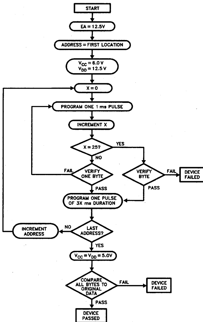
Figure 9. Programming Algorithm
