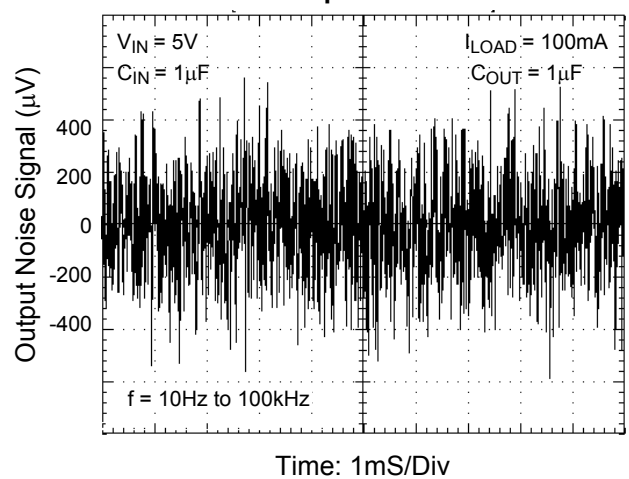
Output Noise
