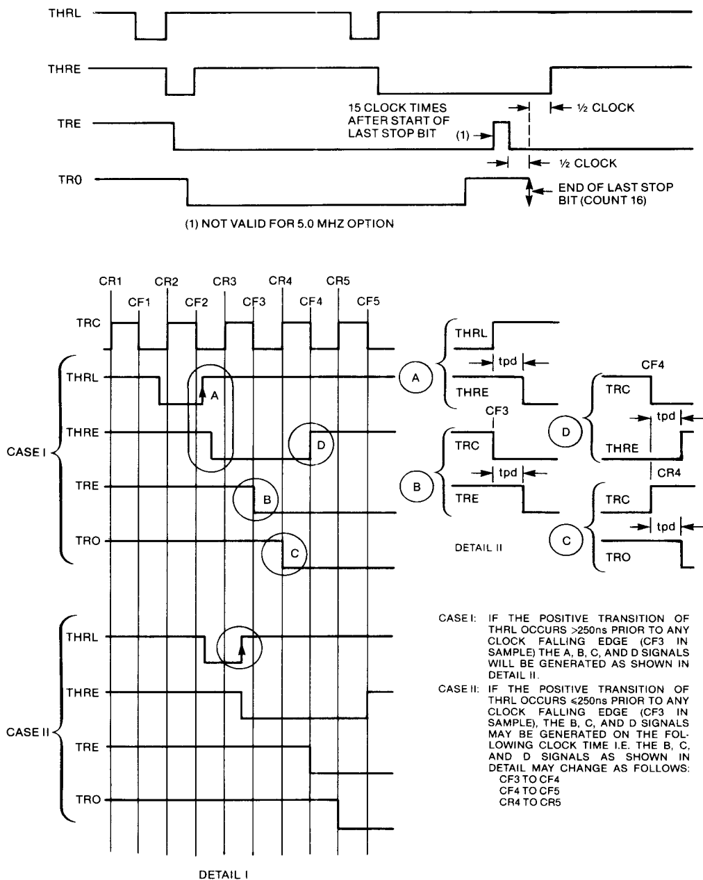
TRANSMITTER TIMING
