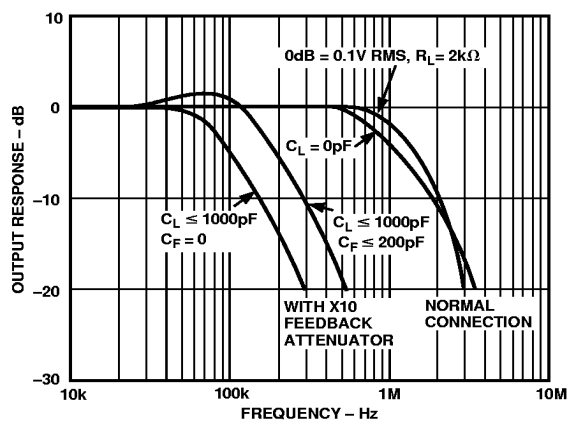
Figure 22. Frequency Response as a Multiplier
