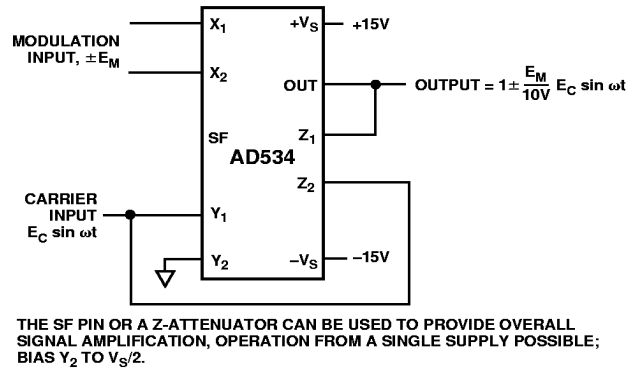
Figure 11. Linear AM Modulator
