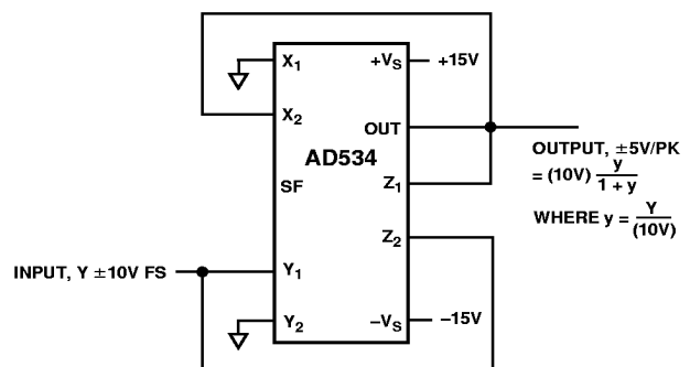
Figure 13. Bridge-Linearization Function
