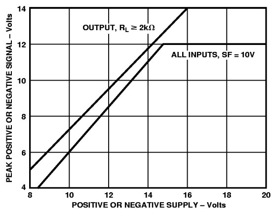
Figure 16. Input/Output Signal Range vs. Supply Voltages
