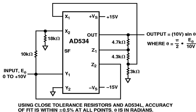
Figure 10. Sine-Function Generator
