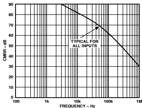
Figure 18. Common-Mode Rejection Ratio vs. Frequency
