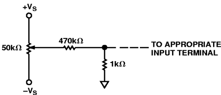
Figure 1. Optional Trimming Configuration
