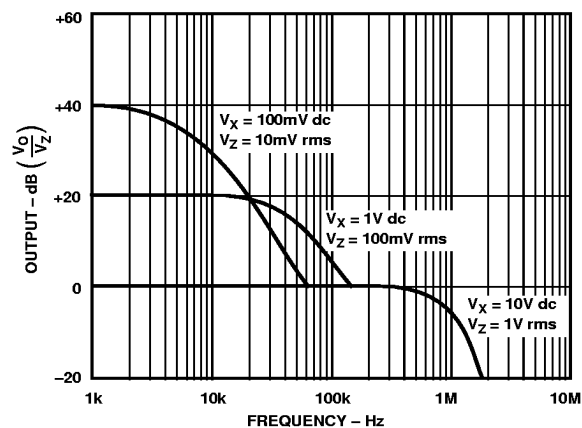
Figure 23. Frequency Response vs. Divider Denominator Input Voltage
