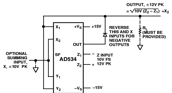
Figure 7. Square-Rooter Connection
