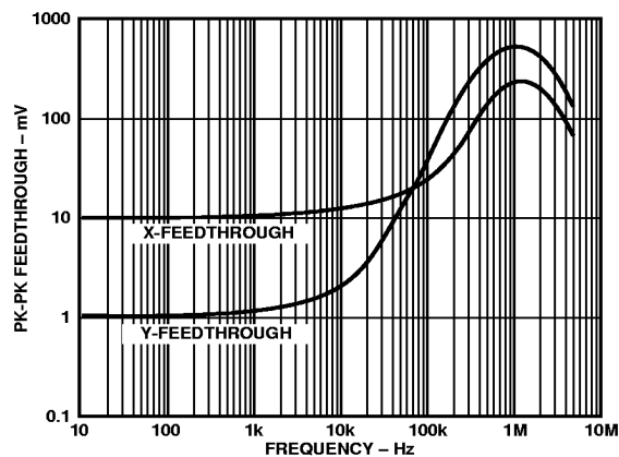
Figure 19. AC Feedthrough vs. Frequency
