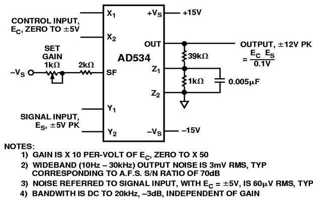
Figure 9. Voltage-Controlled Amplifier
