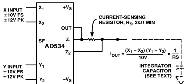
Figure 5. Conversion of Output to Current
