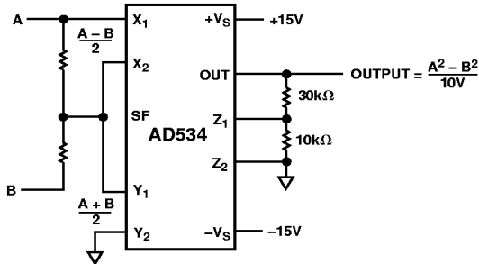
Figure 8. Difference-of-Squares
