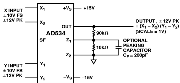
Figure 4. Connections for Scale-Factor of Unity
