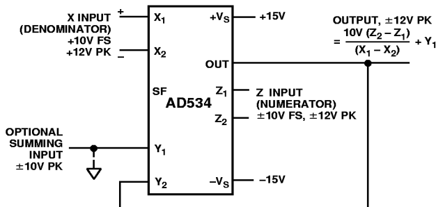
Figure 6. Basic Divider Connection
