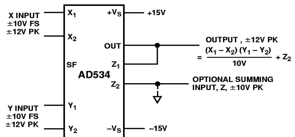
Figure 3. Basic Multiplier Connection
