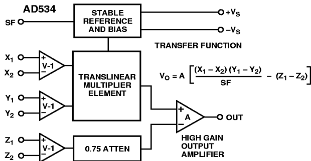
Figure 2. Functional Block Diagram
