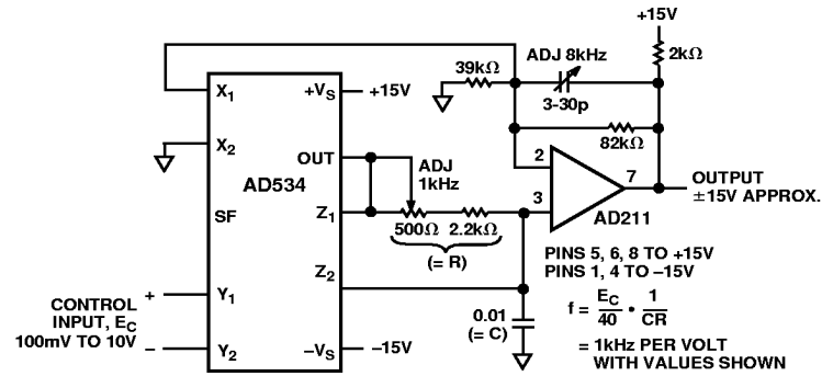
Figure 14. Differential-Input Voltage-to-Frequency Converter
