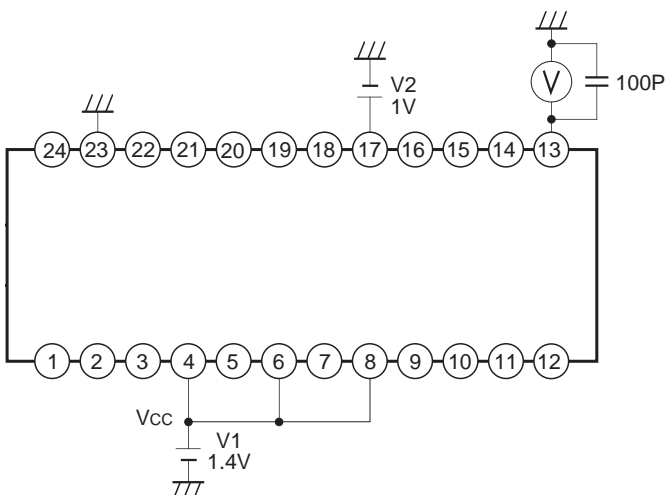
Measurement circuit 10
