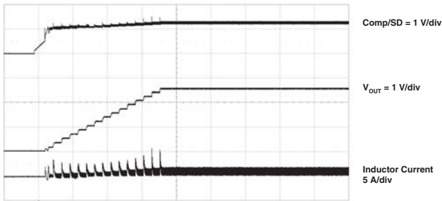
1 \text{ ms/div} V_{IN} = 12 \text{ V} , V_{OUT} = 2.5 \text{ V} , Load Current = 1 A, Output Filter Cap = 220 \mu\text{F} \times 2 Soft Start
