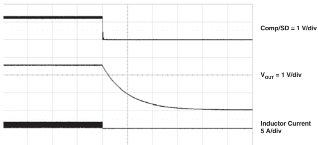
1 \text{ ms/div} V_{IN} = 12 \text{ V} , V_{OUT} = 2.5 \text{ V} , Load Current = 1 A, Output Filter Cap = 220 \mu\text{F} \times 2 Shut Down
