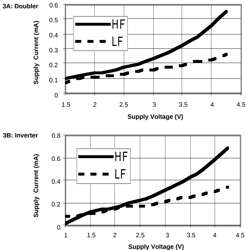
Figure 3A and 3B Supply Current vs. Supply Voltage
